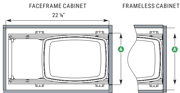
SINGLE WASTEBIN PULLOUT
