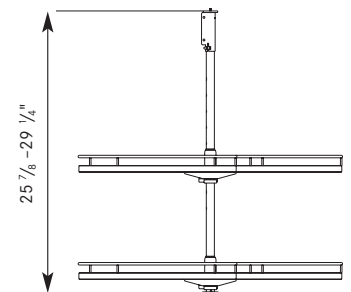
HEIGHT ADJUSTABLE POST
